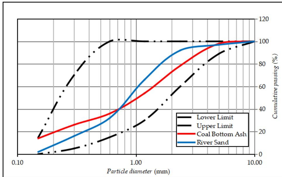
Figure 1. Gradation profiles of CBA and river sand.
